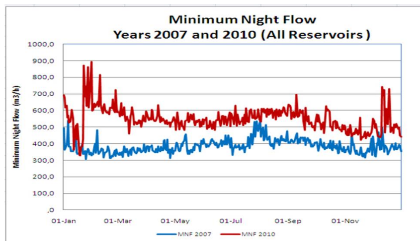
Figure 4 Minimum Night Flow before and after IWS
